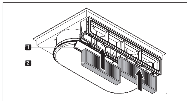
Fig. 5.15 Inserting the activated charcoal filter
