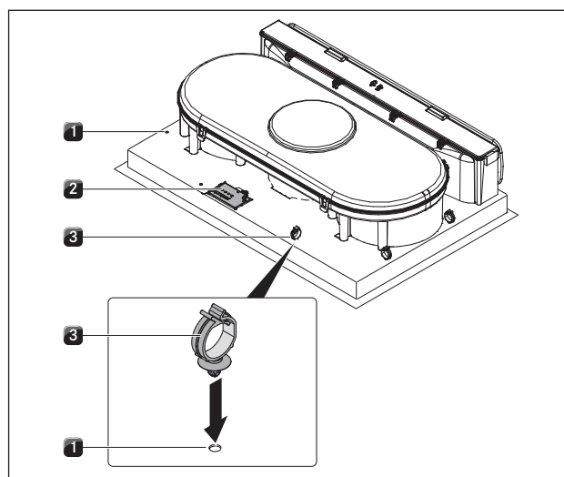
Fig. 5.24 Electrical connections of the cooktop
