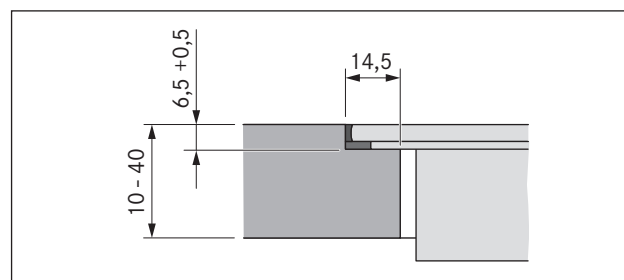
Fig. 5.8 Rebate dimensions for flush installation
