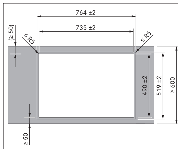
Fig. 5.7 Cut-out dimensions for flush installation
