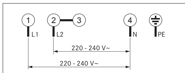
Fig. 5.22 Connection diagram 2-phase connection
