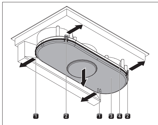
Fig. 12.3 Opening the air guiding housing.
