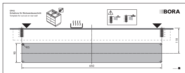
Fig. 5.6 Template for back panel cut-out
