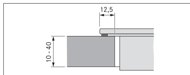
Fig. 5.10 Overlay dimensions for surface mounting
