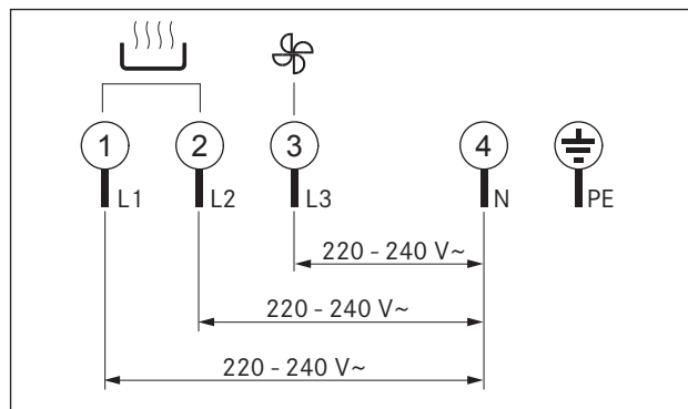
Fig. 5.21 Connection diagram 3-phase connection
