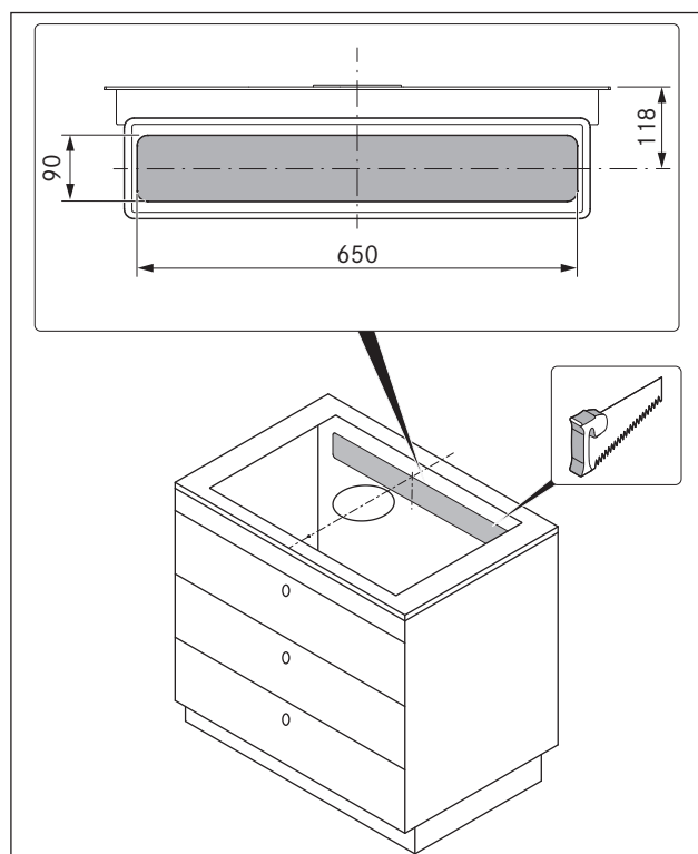
Fig. 5.5 Rear wall cut-out
