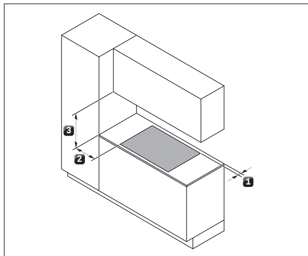
Fig. 5.1 Minimum distance
