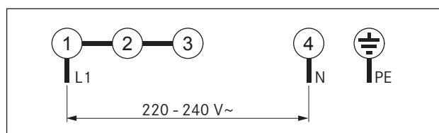
Fig. 5.23 Connection diagram 1-phase connection
