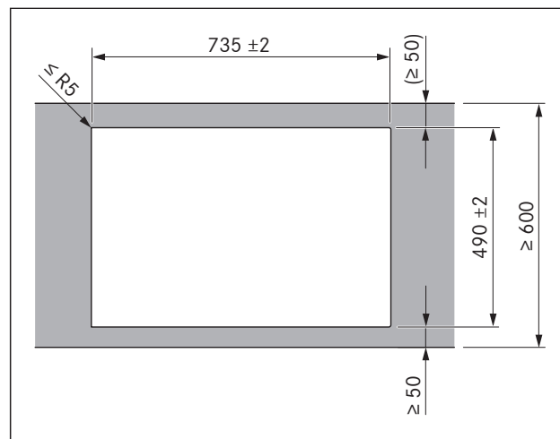
Fig. 5.9 Cut-out dimensions for surface mounting
