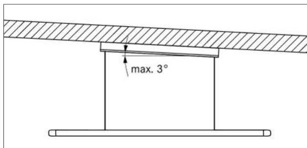
Fig. 5.1 Monteringshelling
