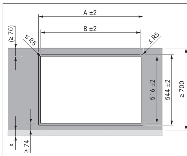
Fig. 5.3 Cut-out dimensions for flush installation
