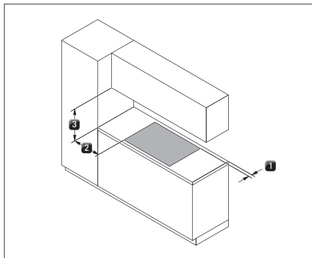
Fig. 5.1 Minimum distance
