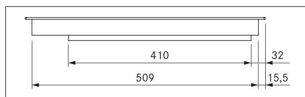
Fig. 3.4 PKI11 Device dimensions side view
