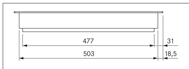
Fig. 3.4 PKT11 Device dimensions side view
