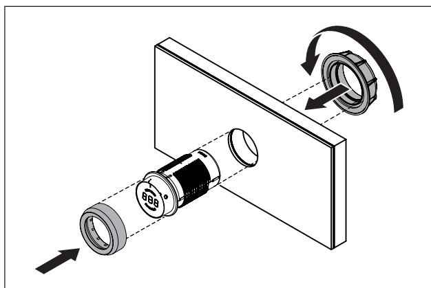
Fig. 5.10 Fitting the control knob
