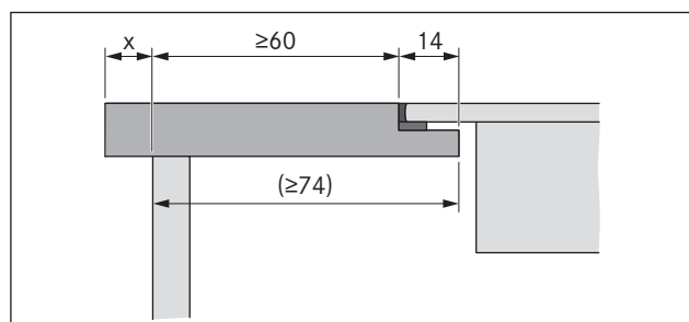
Fig. 5.2 Worktop overhang
