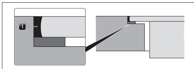
Fig. 5.24 Silicone sealant for flush installation
