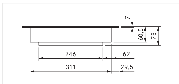
Fig. 3.3 PKT11 Device dimensions front view
