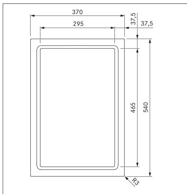
Fig. 3.2 PKT11 Device dimensions aerial view
