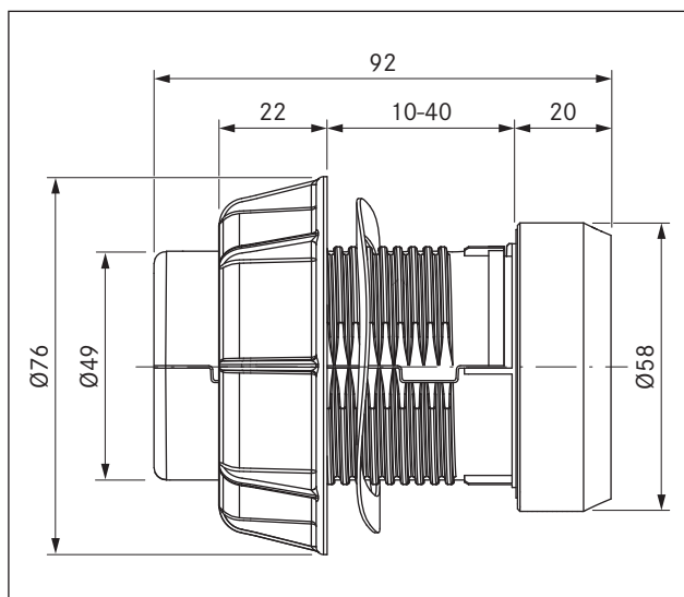
Fig. 3.1 Device dimensions control knob
