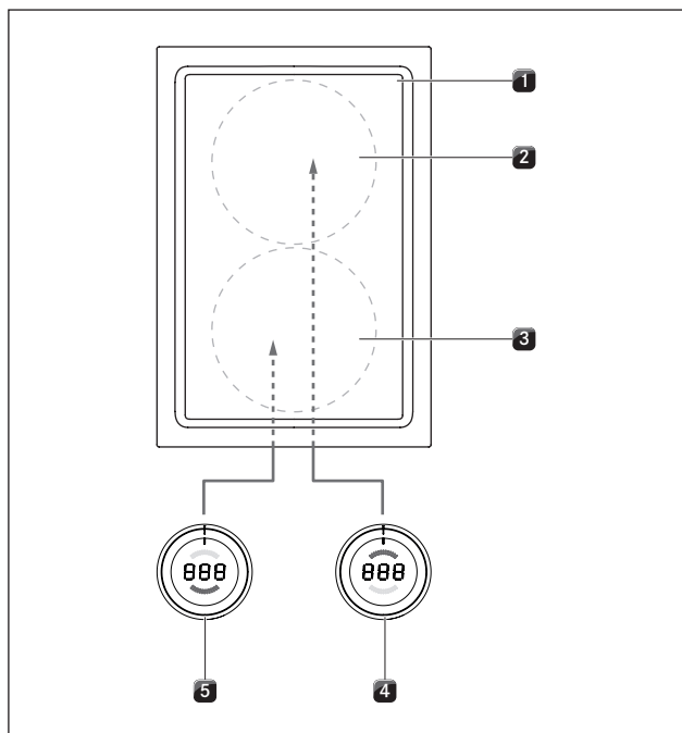
Fig. 5.20 Cooking zone connection in 180° installation
