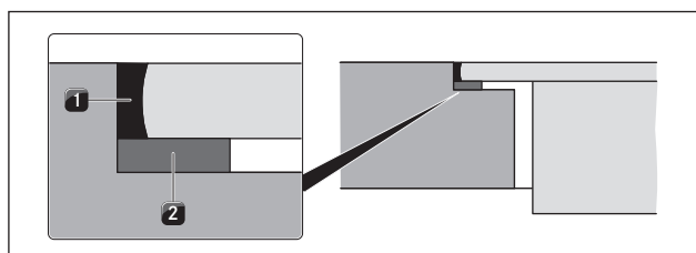
Fig. 5.7 Sealing tape with flush installation
