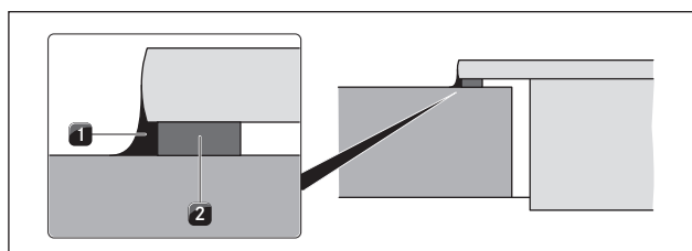
Fig. 5.8 Sealing tape with surface mounting
