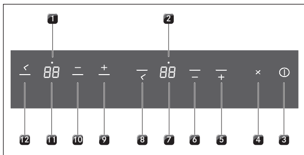
Fig. 4.2 Operating panel
